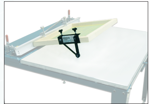
Each unit comes standard with the Big Gripper2 Screen Frame Clamping Unit and a heavy-duty, reversible Side Kick™.
